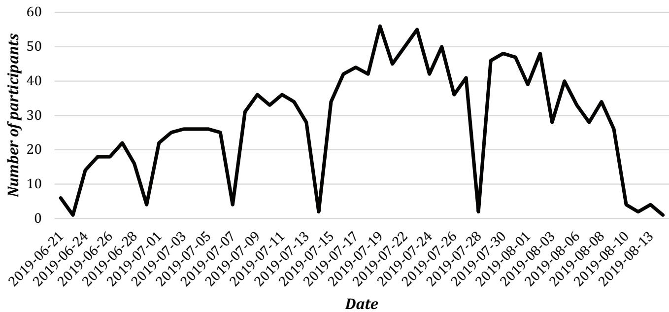
Figure 1. Overall daily enrollment
