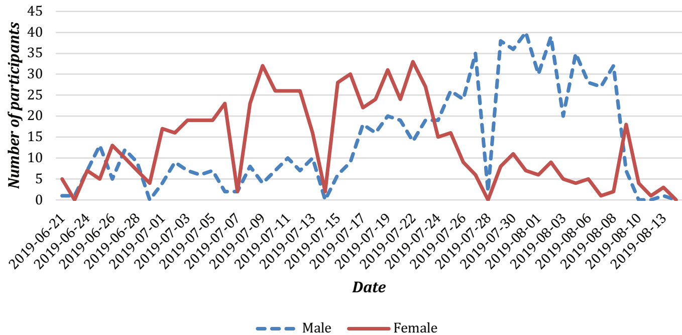
Figure 2. Daily enrollment by gender
