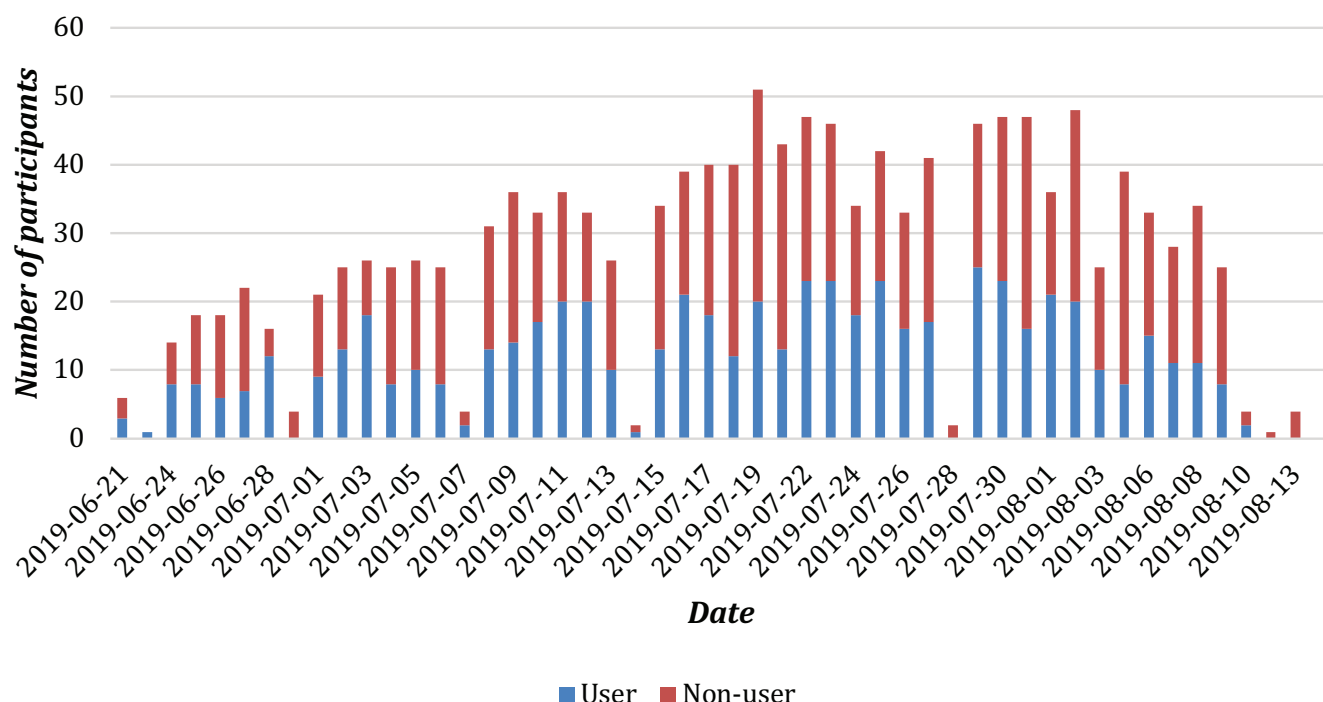
Figure 4. Daily enrollment by participant's reported use of modern contraception
