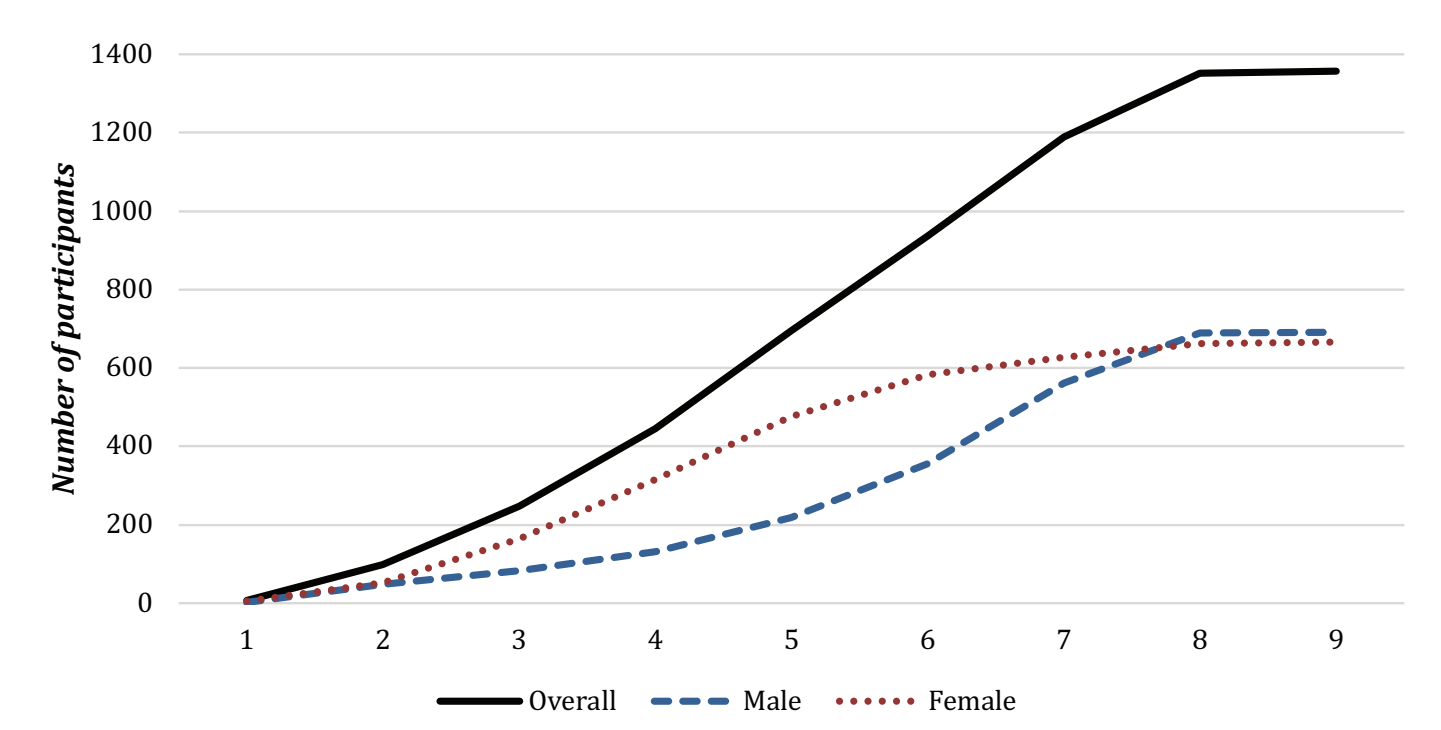
Figure 3. Cumulative weekly enrollment overall and by gender
